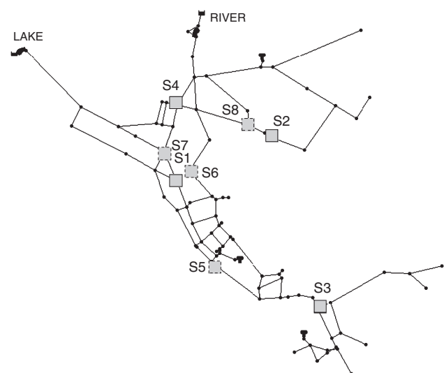
Figure 2 | Water distribution network schematic (small network example). Squares designate sensor locations. For Scenario 1, the sensor network is composed of S1, S2, S3 and S4, Scenario 2 incorporates S1 and S3, only sensor S3 is incorporated in Scenario 3 and Scenario 4 includes S5, S6, S7 and S8.
