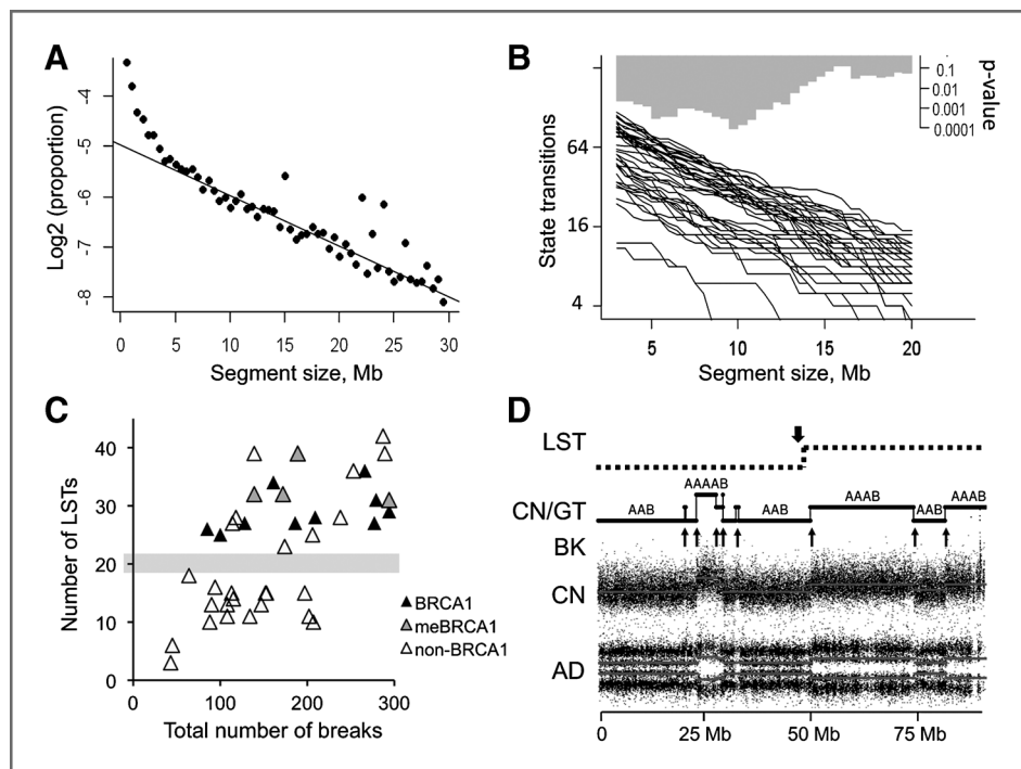
Figure 2. LST number as a surrogate measure of genomic instability A, proportion of segments equal or greater than a given segment size, averaged for the series of 65 BLCs. A linear model was fitted starting from 4 Mb segment size and excluding outliers (values at 15, 22, and 24 Mb were more frequent because of the size of the 18p, 17p, and 19p chromosome arms, respectively). B, number of state transitions depending on the size of the segments; each line corresponds to a near-tetraploid BLC; significance profile for BRCA1 versus non- BRCA1 tumors comparison is shown on the top of the plot. C, genomic instability in near-tetraploid BLCs as estimated by the total number of breaks and by LSTs (segment size 10 Mb). LST number clearly discriminated non- BRCA1 BLCs from BLCs with proven BRCA1 inactivation ( P < 0.001 , Wilcoxon test). Total number of breaks was less significantly different between non- BRCA1 versus BRCA1 and me BRCA1 comparison ( P < 0.03 , Wilcoxon test) and was not discriminative. BRCA1 , germline BRCA1 mutation; me BRCA1 , BRCA1 promoter methylation; non- BRCA1 , absence of evidence of BRCA1 inactivation. D, an example of genomic profile with 1 LST detected. CN, copy number profile; AD, allelic difference profile; CN/GT, segmental copy numbers and genotypes recognized by GAP; BK, total breaks; LST, large-scale state transition. The dashed line shows large-scale segments obtained after filtering and smoothing small-scale variations seen in the CN/GT profile.
