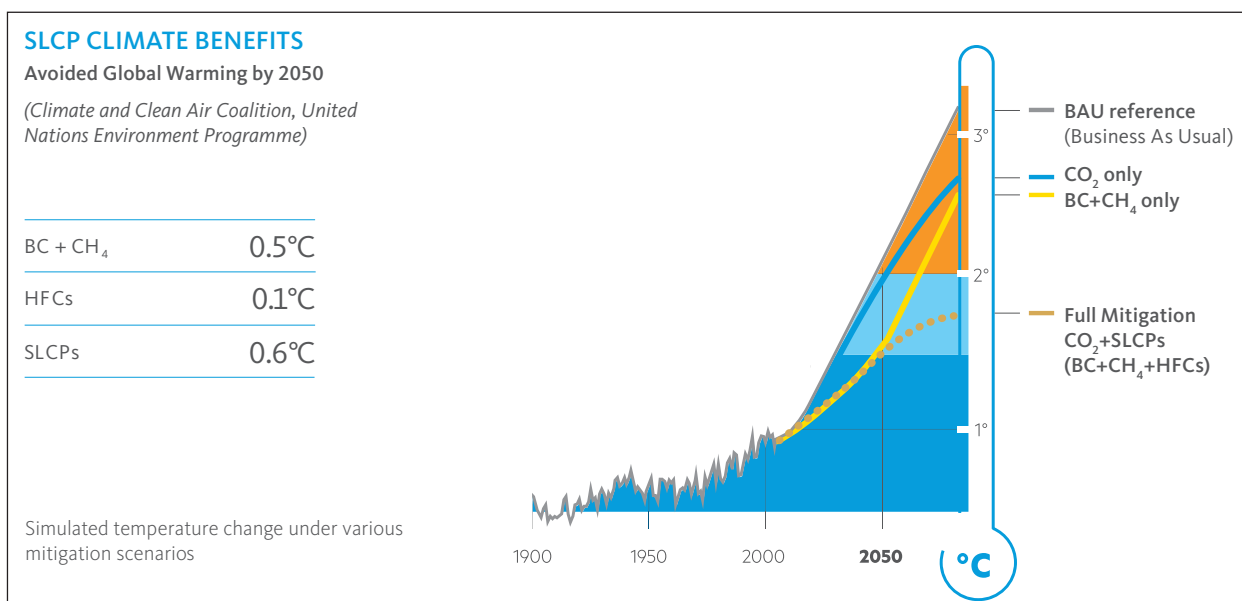
Figure 2: Simulated temperature change under various mitigation scenarios and SLCP Climate benefits.
