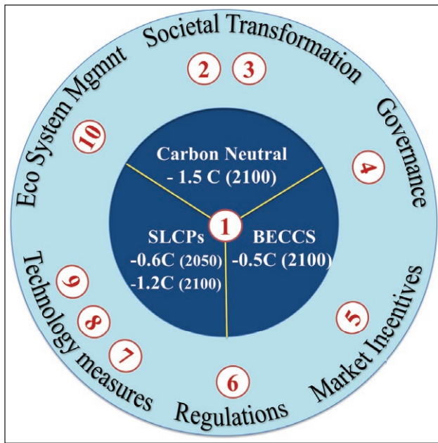
Figure 1: Ten Solutions to Bend the Curve and Limit Warming to Under 2°C.
