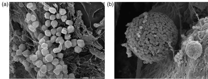
Figure 6 | FeS 2 formation in the interstices (5–6 cm depth) at Lake Tegel bank filtration site. (a): Beginning anaerobic conditions with distinct FeS 2 crystals covering the extracellular polymeric substances (EPS), which form net structures and plaques (right side, above). (b): Matured FeS 2 crystals as framboidal pyrite formed in the EPS. SEM photos; crystal determination by SEM-EDS.
