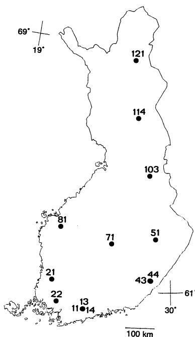
Fig. 1. Location of the 13 research drainage basins. The numbers refer to those in Table 1.
