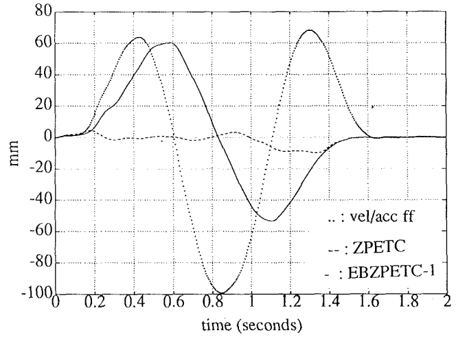
Fig. 6 Comparison of end point tracking errors using velocity and acceleration feedforward, ZPETC, and EBZPETC-1
