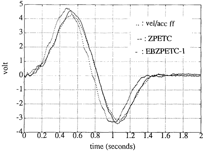
Fig. 5 Comparison of input signals to the motor using velocity and acceleration feedforward, ZPETC, and EBZPETC-1
