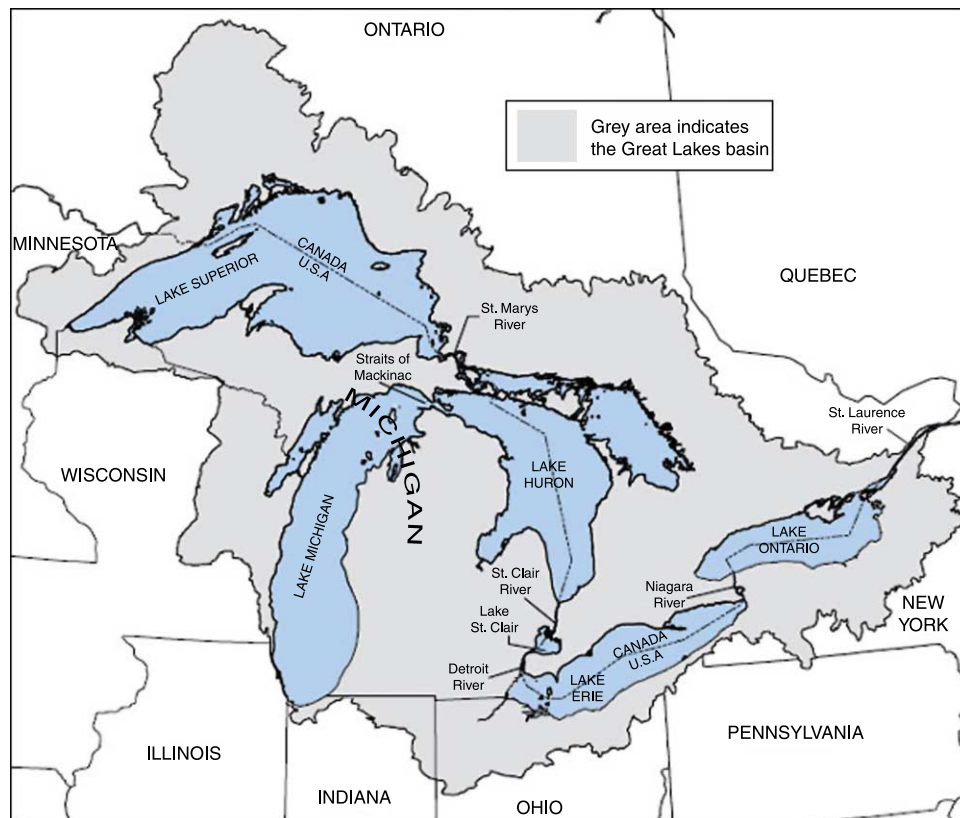
Figure 1 | The Great Lakes basin in North America.
