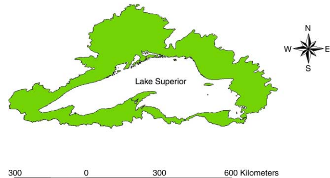
Figure 2 | Lake Superior and its surrounding watersheds.
