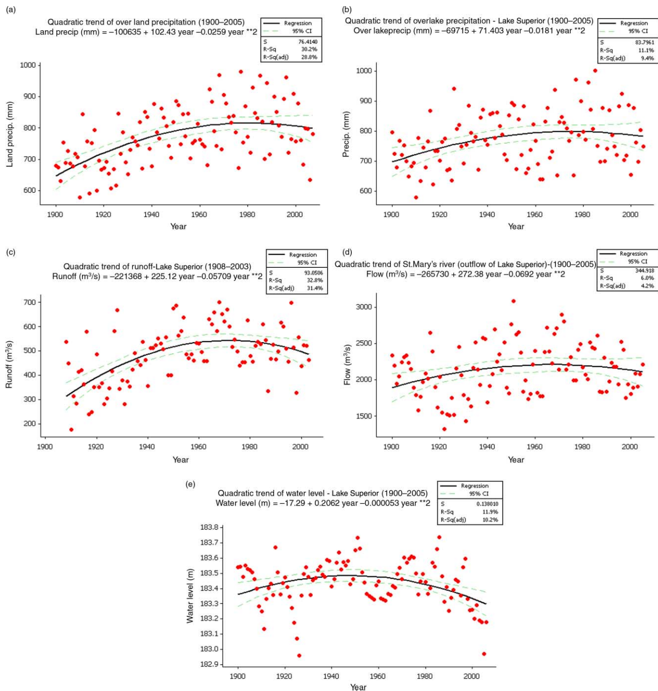
Figure 6 | Quadratic trends for average annual (a) land precipitation, (b) overlake precipitation, (c) runoff, (d) outflow and (e) water level for Lake Superior (1900–2005).
