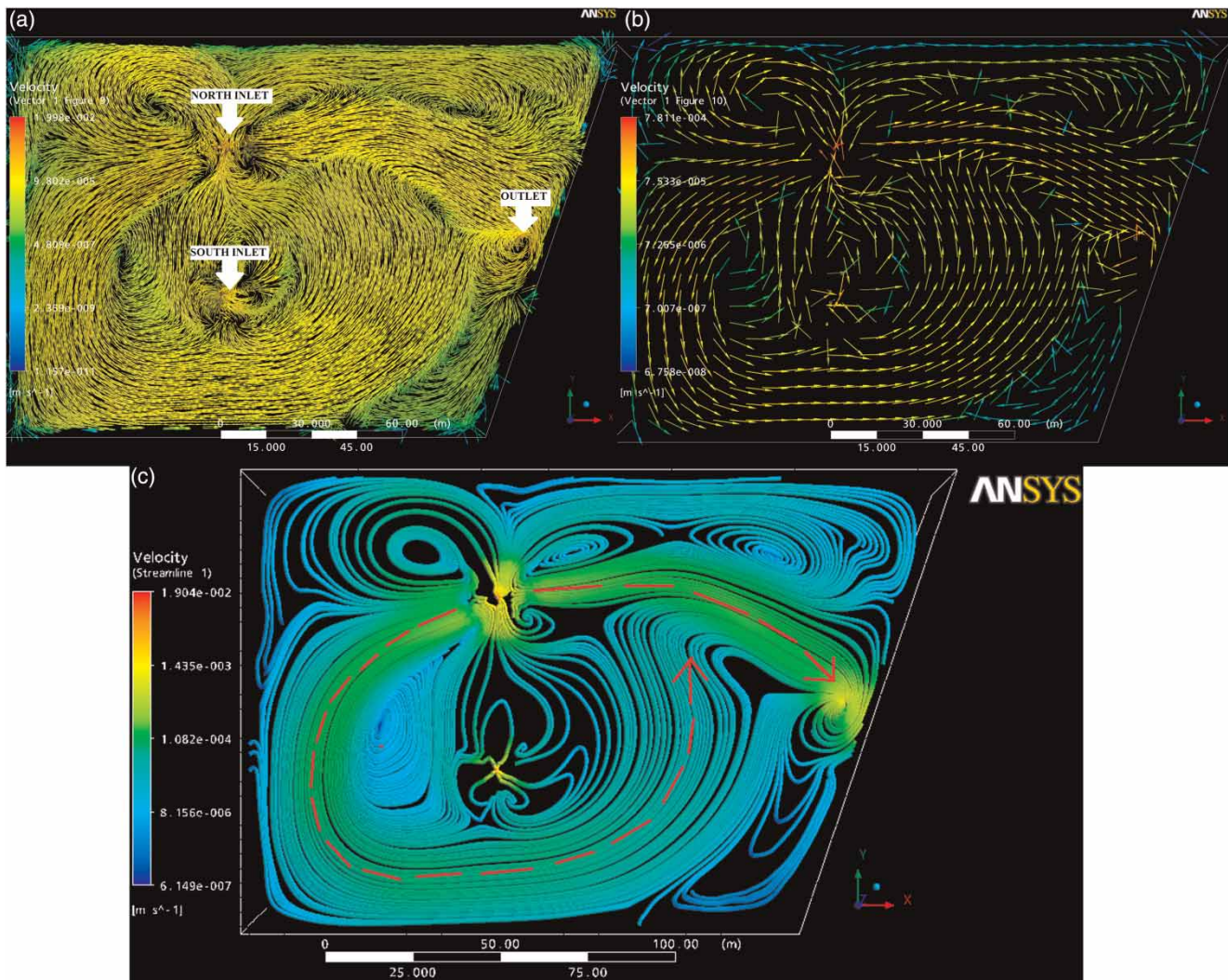
Figure 2 | (a) Three-dimensional velocity vectors obtained with the CFD model in the facultative pond – XY plane in Z = 1.70 m, (b) velocity vectors uniformly distributed in the facultative pond – XY plane in Z = 1.70 m and (c) stream lines in the facultative pond – XY plane in Z = 1.70 m.
