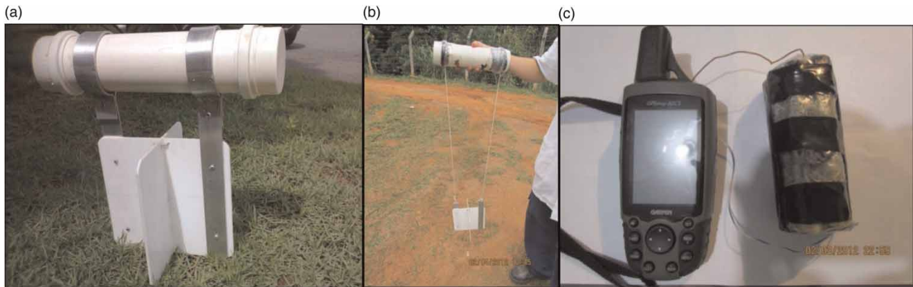
Figure 1 | (a) Prototype of the drogue mounted to record the flow in the pond, (b) modified drogue with adjustable length, to follow the flow at any depth in the ponds, and (c) GPS and battery adapted for use in the drogue.
