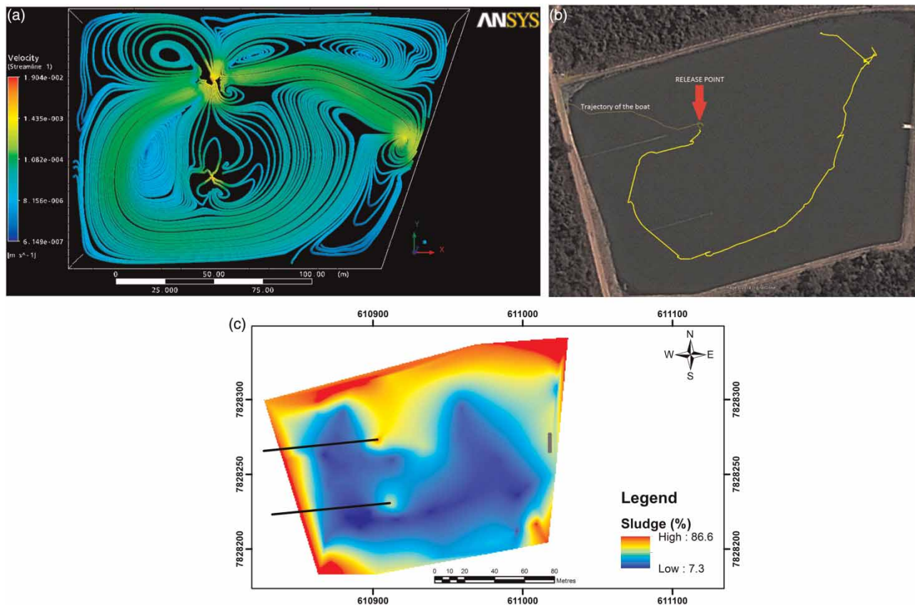
Figure 3 | Comparison between (a) the flux lines obtained by modelling, (b) the path obtained with the drogue and (c) the map of sludge accumulation, expressed as percentage of the net pond depth – from 7.3 to 86.6% (Passos et al. 2013).
