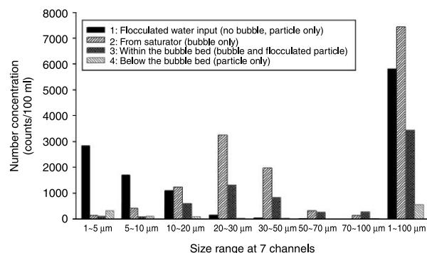
Figure 7 | Particle and bubble count data at various locations in the DAF process (case 2).
