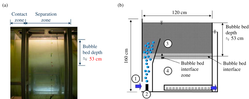
Figure 1 | Pilot plant used to determine the bubble bed depth: (a) pilot plant manufactured from transparent acrylic; (b) cross-section of pilot plant.
