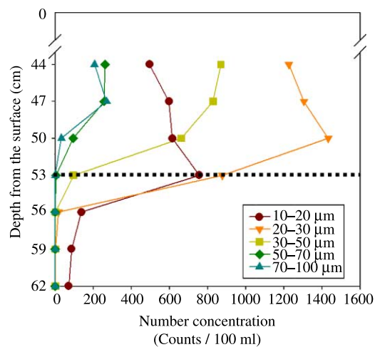
Figure 3 | Particle and bubble counts with depth in a pilot plant (operating conditions: pressure, 517 kPa; recycle ratio, 50%, separation zone loading rate, 1.4 m h -1 ; water temperature, 7.5°C).
