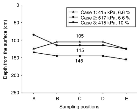
Figure 6 | Change of bubble bed depth at different operating conditions (operating conditions: separation zone loading rate, 12 m h -1 ; water temperature, 7.5°C).
