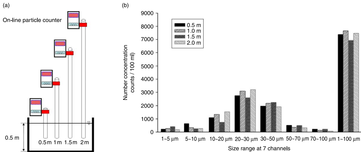
Figure 8 | The effect of length of sampling tubes (internal diameter, 3 mm) in a continuous reactor: (a) experimental setup with sampling tube and particle counter; (b) bubble size distribution.
