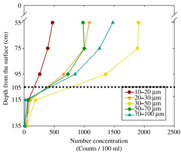
Figure 4 | Particle and bubble count at different depths at sampling position C (operating conditions: pressure, 415 kPa; recycle ratio, 6.6%; separation zone loading rate, 12 \text{ m h}^{-1} ; water temperature, 7.5^\circ\text{C} ).
