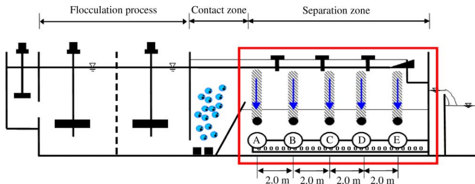
Figure 2 | Schematic diagram and sampling points at Wonju DAF plant.
