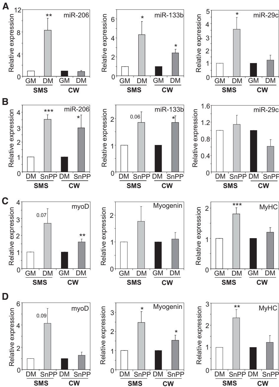
Figure 4. Expression of differentiation markers in SMS-CTR (eRMS) and CW9019 (aRMS) cell lines cultured in differentiation medium (DM) with or without SnPP (10 \mu mol/L, 5 days). A , expression of miR-206, miR-133b, and miR-29c in cells cultured in differentiation medium. N = 6-26 . B , effect of SnPP on expression of miR-206, miR-133b, and miR-29c in cells cultured in differentiation medium. N = 2-16 . C , expression of myoD, myogenin, and MyHC in cells cultured in differentiation medium. N = 10-27 . D , effect of SnPP on expression of myoD, myogenin, and MyHC in cells cultured in differentiation medium. N = 3-11 . Quantitative RT-PCR. U6 ( A and B ) and EF2 ( C and D ) served as internal control. *, P < 0.05 ; **, P < 0.01 ; ***, P < 0.001 versus growth medium (GM; A and C ) or control differentiation medium ( B and D ). Values of P < 0.1 are indicated.
