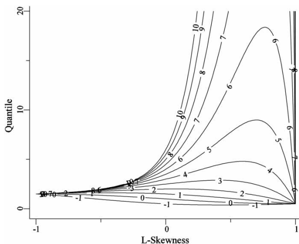
Figure 2 | Anomalous behaviour of the quantiles of a distribution. Showing quantiles of a generalised logistic distribution with fixed first and second L-moments as the L-skewness varies. Each line is for a different return period and is labelled with the corresponding Gumbel reduced variate.
