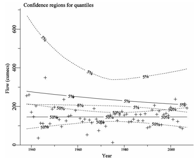
Figure 3 | Central estimates and 90% confidence regions (dashed lines) for flows having 50 and 5% exceedance probabilities in the given year. Showing annual maxima for Day’s weir 1938–2007.
