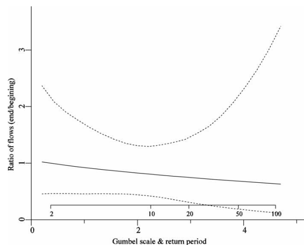
Figure 4 | Central estimate and 90% confidence region (dashed lines) for the ratio defined by the flow of a given return period in 2007 divided by the flow of the same return period in 1938.
