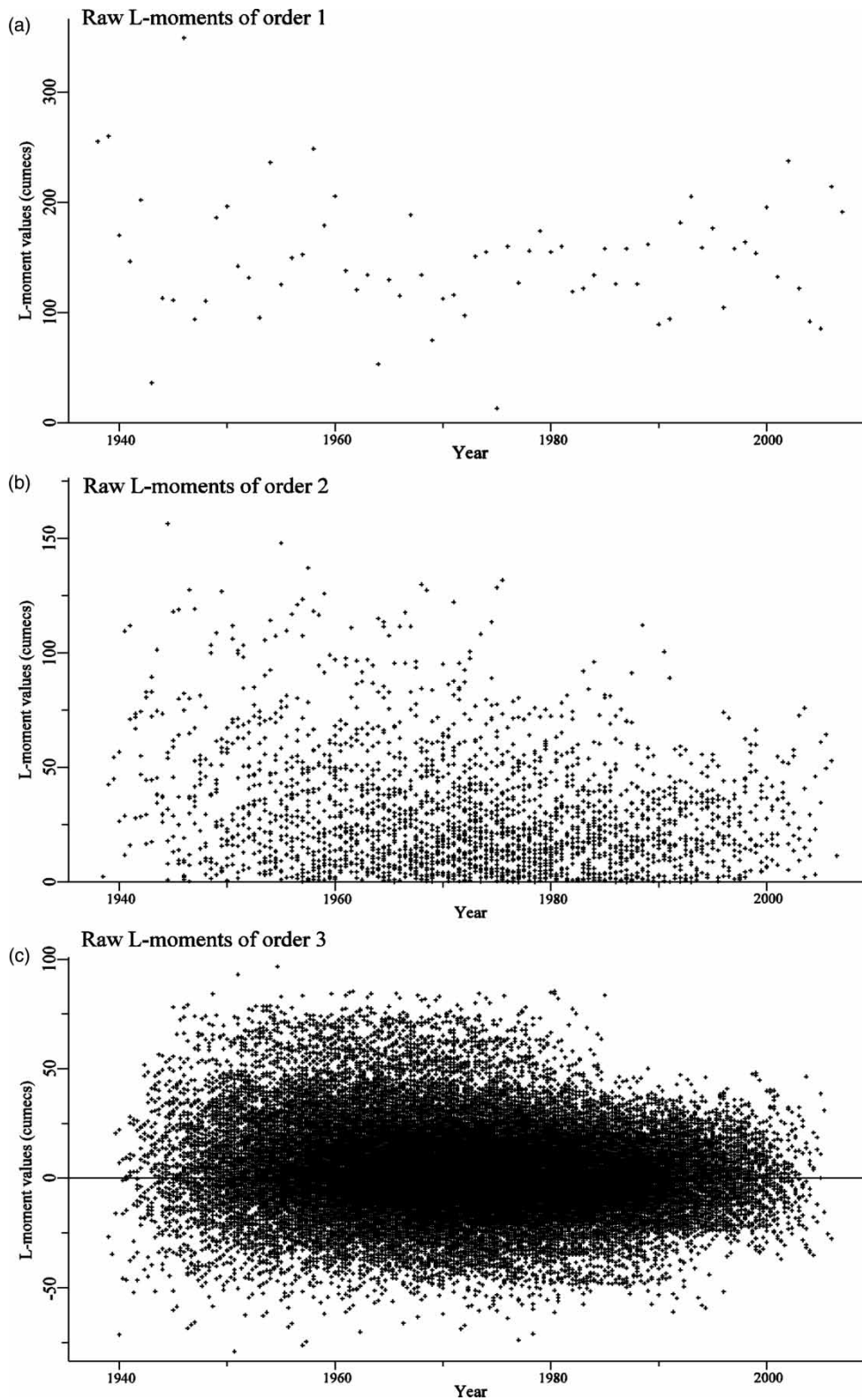
Figure 1 | Raw L-moments of orders 1, 2 and 3, plotted at average time-points. Data are annual maxima for Day's weir 1938–2007.
