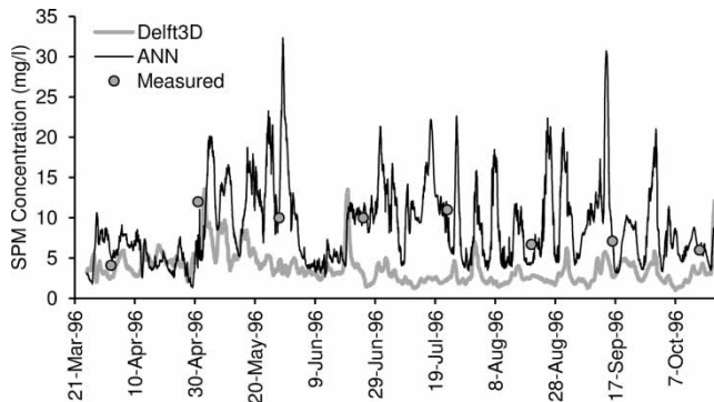
Figure 8 | SPM concentrations predicted by the ANN model and by the numerical model based on Delft3D together with the measured SPM concentrations at IJmuiden.
