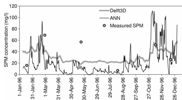
Figure 7 | SPM concentrations predicted by the ANN model (after correction) and by the numerical model based on Delft3D together with the measured SPM concentrations at Schouwen.
