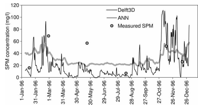
Figure 7 | SPM concentrations predicted by the ANN model (after correction) and by the numerical model based on Delft3D together with the measured SPM concentrations at Schouwen.
