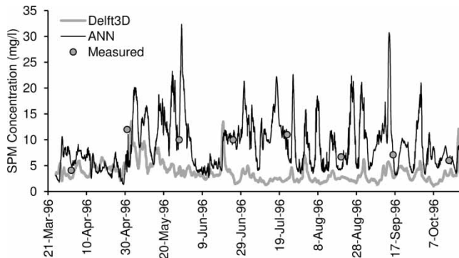
Figure 8 | SPM concentrations predicted by the ANN model and by the numerical model based on Delft3D together with the measured SPM concentrations at IJmuiden.
