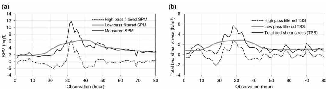
Figure 2 | (a) Variation of suspended particulate matter (SPM) concentration at 10 km offshore of Noordwijk for a storm during 16–19 May 2001 along with the low pass and high pass filtered SPM concentration for the same storm. (b) Variation of total bed shear stress at 10 km offshore of Noordwijk for the same storm period of (a) along with the low pass and high pass filtered total bed shear stress.
