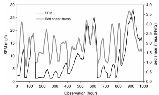
Figure 4 | Variation of filtered SPM and filtered bed shear stress for multiple storms.
