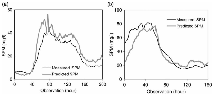
Figure 6 | Comparison of SPM concentration predicted by the ANN model with the measured data for Noordwijk-2. (a) During a storm period during 29 September 2001 to 7 October 2001 (about a week). (b) During another storm period during 20–27 November 2001 (about a week).
