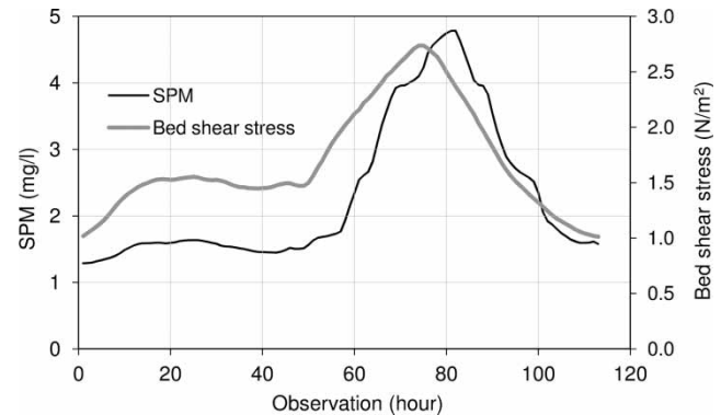
Figure 3 | Variation of low pass filtered suspended particulate matter (SPM) concentration along with low pass filtered total bed shear stress at 10 km offshore of Noordwijk for a storm during 8–13 July 2001.
