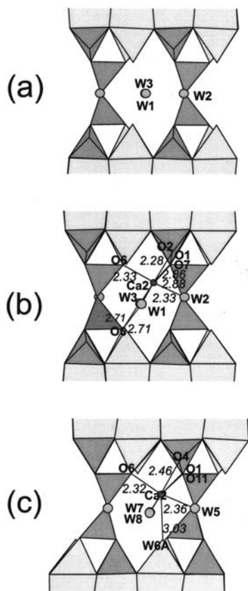
Fig. 9. Schematic drawing of the structural cavities, as seen along [010] in (a) anomalous tobermorite 11Å from Wessels mine; (b) normal tobermorite 11Å from Urals; (c) clinotobbermorite from Wessels mine (Merlino et al. , 2000). In (b) one of the two possible ordered arrangements of Ca2, W1, and W3 is reported.
