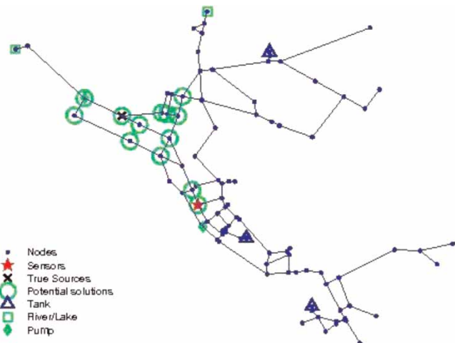
Figure 10 | Potential contamination source locations identified for the one-sensor case (Scenario 7).
