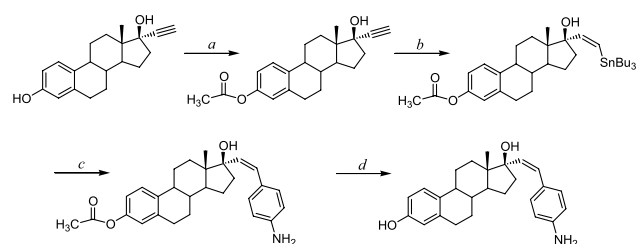
Figure 1. Synthesis of 17 \alpha -Z- p -aminophenylvinyl-17 \beta -estradiol (APVE 2 ). a , 17 \alpha -Ethynyl-E 2 , acetic anhydride, pyridine, room temperature, 12 h; b , 2 , tributyltin hydride, triethyl borane, N 2 , room temperature, 10 h; c , p -iodoaniline, triphenylphosphine palladium (0) in refluxing toluene, 20 min added to 3 , 2,6-di- t -butyl-4-methylphenol, toluene, reflux, N 2 , 17 h; 10% KF/H 2 O, 1 h, room temperature; d , 4 , 10 N sodium hydroxide in methanol, 2 h, room temperature.
