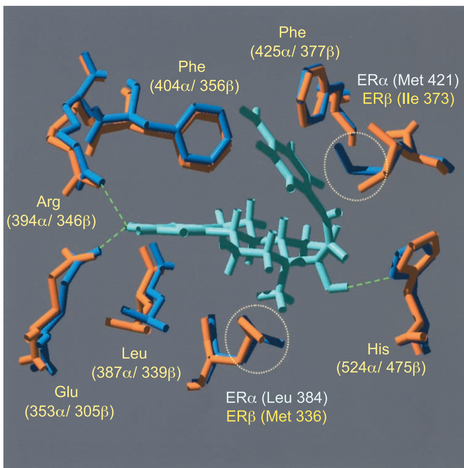
Figure 2. An energy minimized depiction of APVE 2 is shown bound within the ligand binding pocket of ER- \beta (orange) and ER- \alpha (blue). Hydrogen bonds are illustrated as dotted lines. The phenyl moiety was predicted to cause a higher level of steric hindrance within the ligand binding pocket of ER- \alpha as a result of Met421 as opposed to the corresponding Ile373 for ER- \beta .
