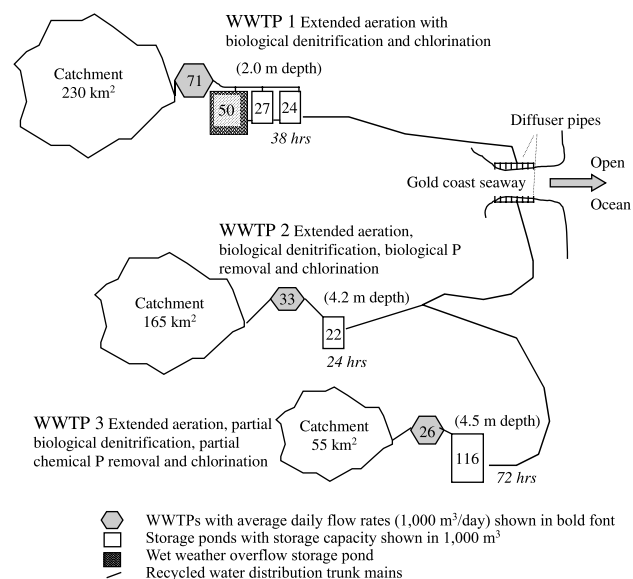
Figure 1 | Wastewater catchments, treatment plants (WWTP 1, 2 and 3) and their recycled water distribution systems on the Gold Coast, Queensland, Australia (retention times in storage ponds shown in italics).
