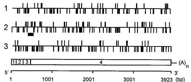
Fig. 4. Open reading frame analysis. The relative positions of ATG codons and termination codons (TGA, TAA, and TAG) are indicated by vertical lines, respectively, for each of the three reading frames. The small black rectangle indicates the most likely open reading frame of DD3 as predicted by Grail software. The four open boxes (□) represent exons 1–4 of the DD3 gene.
