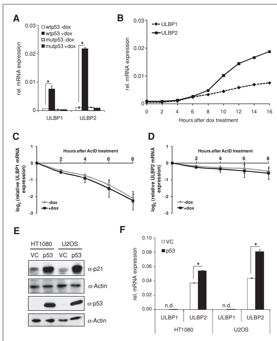
Figure 2. ULBP1 and -2 are upregulated at the transcriptional level. A, expression of ULBP1/2 mRNAs was monitored in wt/mt p53 H1299 cells 16 hours after \pm doxycycline treatment by quantitative real-time PCR. B, kinetics of ULBP1/2 mRNA expression in wtp53 H1299 cells after doxycycline treatment is shown. A and B, ULBP1/2 mRNA expression levels are depicted relative to GAPDH mRNA expression levels (set as 1). The mean of 2 independently conducted experiments \pm SD is shown. C and D, wtp53 H1299 cells were either left untreated or treated for 10 hours with doxycycline, and ULBP1/2 mRNA expression was monitored by quantitative real-time PCR at different time points after the addition of 10 \mu g/mL actinomycin D (ActD). \log_2 of relative ULBP1/2 mRNA expression compared with the relative ULBP1/2 mRNA expression before the addition of ActD (set as 1) is shown. Expression of ULBP1/2 was normalized to GAPDH. E and F, HT1080 and U2OS cells were transfected with either 2 \mu g of a wtp53 expression plasmid (p53) or 2 \mu g of pcDNA3.1+ (VC). E, expression of p53, p21, and actin was analyzed by Western blot 24 hours after transfection. F, relative ULBP1/2 mRNA expression 24 hours after transfection was monitored as described in (A, B). B–F, one representative experiment of 2 independently conducted experiments is shown. The mean of duplicates \pm SD is depicted. *, P < 0.05 determined by Student's t test; n.d. = not detectable; VC = vector control; dox, doxycycline.
