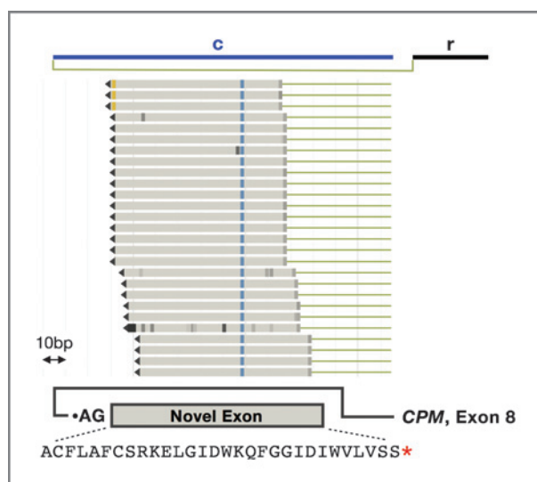
Figure 3. Novel CPM C-terminal exon expressed from the TCGA-06-0648 double minute chromosome. The top line shows the appropriate region from Fig. 1C, with sequencing reads where the other pair maps to exon 8 of CPM below. The bottom panel shows the orientation of the new exon relative to CPM and its amino acid sequence.
