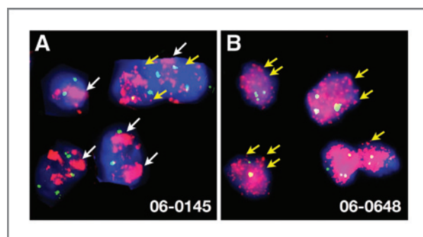
Figure 4. Visualization of glioblastoma multiforme tumor oncogenic amplicons. FISH analysis of formalin-fixed paraffin-embedded blocks matching samples 06-0145 (A) and 06-0648 (B). Probes for the centromeric region of chromosome 7 (A) and chromosome 12 (B) shown in green gave two to four foci per cell. Probes for EGFR (A) and MDM2 (B) are shown in pink. White arrows point to broad, HSR-like staining patterns, and yellow arrows point to discrete extrachromosomal spots.
