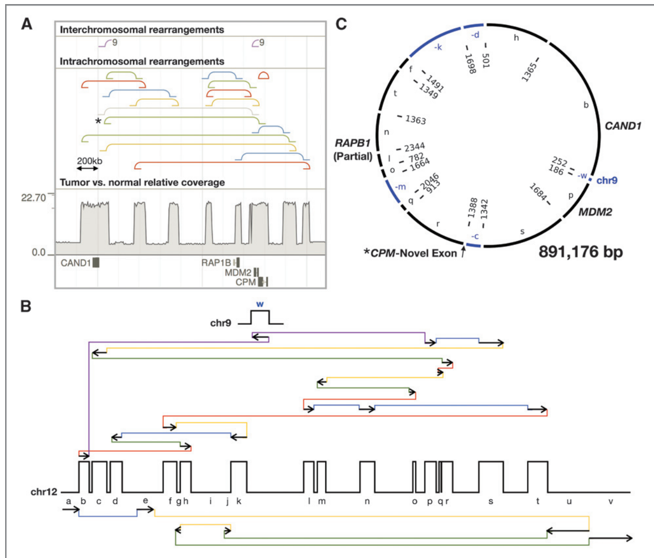
Figure 1. Reconstruction of TCGA-06-0648 double minutes. A , tumor browser view of a region of chromosome 12 from TCGA-06-0648. The bottom track shows protein-coding genes overlapping the amplified segments. The track above shows relative copy number of the tumor DNA compared with the normal, showing distinct blocks of elevated copy number with similar total copy number between blocks. The next two tracks show intra- and interchromosomal rearrangement breakpoints. All rearrangements shown are supported by at least 100 discordant reads. The type of rearrangement is indicated by the color of the line: duplication (red), deletion (blue), inversion (yellow and green), and interchromosomal rearrangement (purple). B , a diagram of the amplified segments and structural variants identified on chromosome 12 and 9 is shown. Walking through this diagram results in a circular solution, suggesting the double minute chromosomes diagrammed in C where segments inverted relative to their orientation in the reference genome are indicated by (-) and colored blue. The letters inside the circle correspond to the segments in B . The numbers inside the circle indicate the number of sequencing reads supporting each breakpoint.
