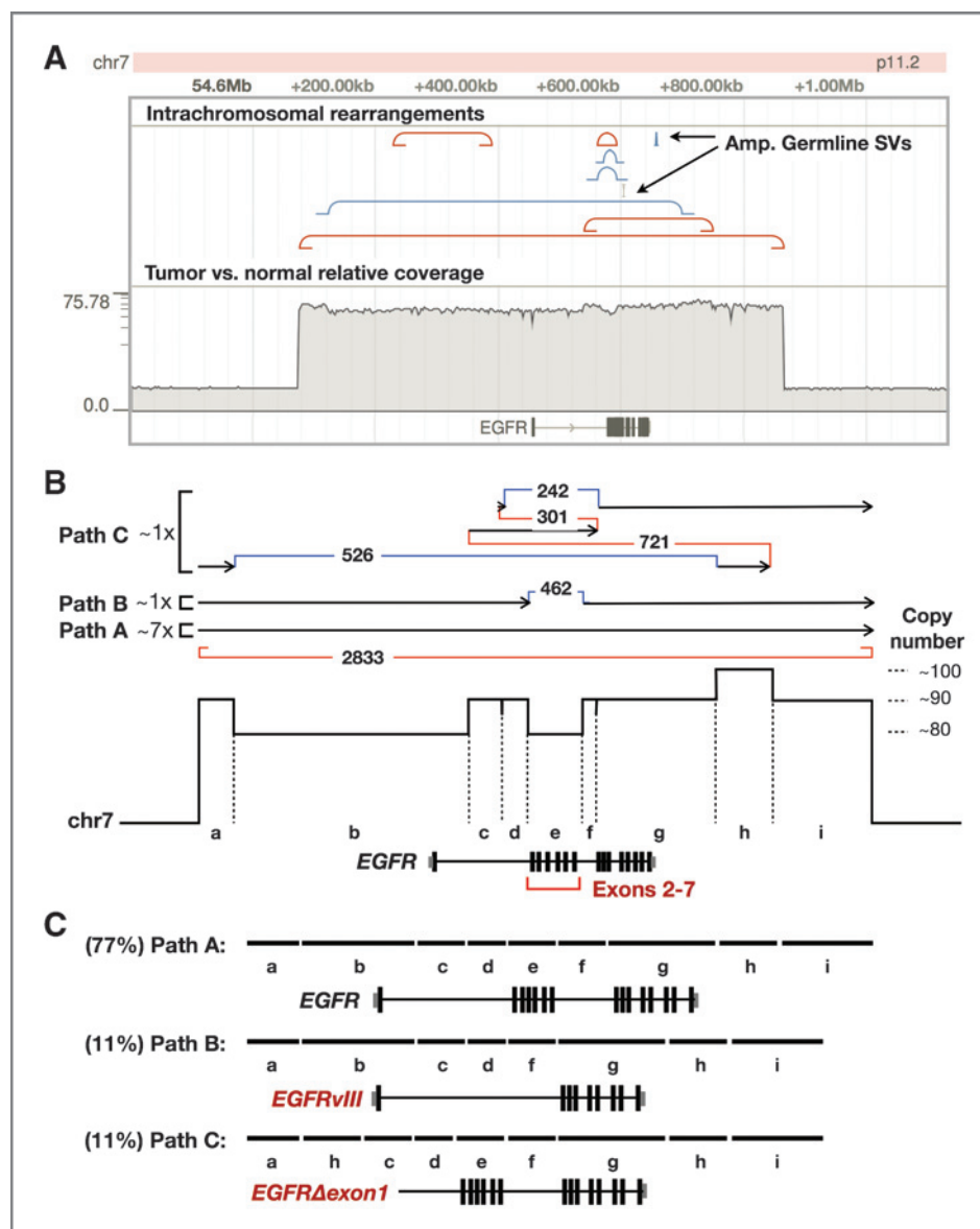
Figure 2. Reconstruction of 06-0145 amplicons. A, browser shot of the amplicon on chromosome 7. Tracks as described for Fig. 1. The two "Amp. Germline SVs" are known germline breakpoints present on the amplicon. B, diagram of the three paths that together form a potential solution of the breakpoint graph for sample TCGA-06-0145 that accounts for all observed, highly supported breakpoints. The location of the gene EGFR is noted. Note that all paths, A, B, and C, can create circular solutions by using the encompassing tandem duplication shown in red to connect the end of each path to the beginning. The tandem duplication may also connect path A to path B, path C to path B, and so on. C, the effects of each path on the EGFR gene, showing that path B creates an oncogenic form of EGFR , EGFRvIII , through specific deletion of exons 2 to 7.
