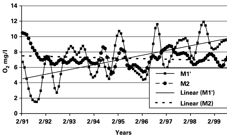
Figure 6 Trend cycles of decomposed dissolved oxygen time series of the Musa river streamwater at the reaches M1' (6.4 km below the Kulpe tributary) and M2 (after self-purification of running water, fixed at 91.5 km below the Kulpe tributary)
