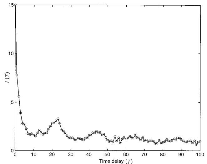
Figure 11 | Average mutual information function for the residual Venice Lagoon data from 1980–1989. I(T) has its first minimum at T=8 hours.
