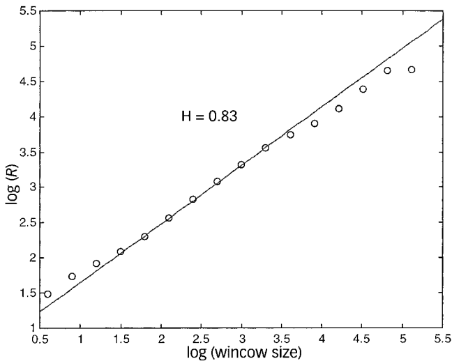
Figure 5 | Estimation of the Hurst coefficient for the level data from Figure 1. Selected points have been excluded from the calculation (see Cannon et al. 1997, Table 2).
