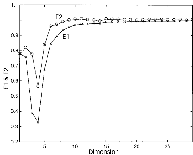
Figure 15 | E1 & E2 method for the level data at Venice Lagoon 1980-1994.
