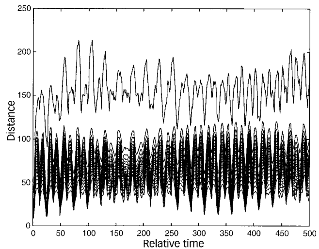
Figure 7 | Space-time separation plot of the Venice Lagoon level data. Lines of constant probability density of a point to be e-neighbour of the current plot if its temporal distance is \delta t (relative time) are shown. Probability densities are 1/20 to 1 with increments of 1/20 from bottom to top. Clear correlations are visible (calculations were carried out using the stp routine of the TISEAN package, http://www.mpi-pks-dresden.mpg.de/~tisean ).
