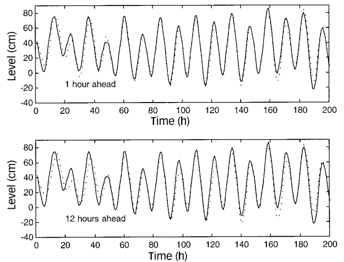
Figure 21 | Observed (continuous) and predicted (dashed) water level values from Venice Lagoon, 1 and 12 hours forecasting. The predictions were made using local linear polynomial predictors whose coefficients were learned from 68,000 data points. These were embedded in d_E=8 using a d_L=8 dimensional model.
