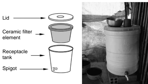
Figure 2 | Ceramic filter.
