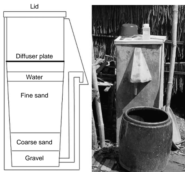
Figure 1 | BioSand filter.
