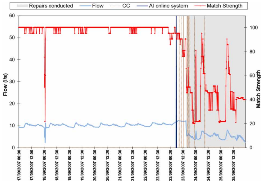
Figure 6 | AURA Alert Match Strength and supporting information for potential precursor.
