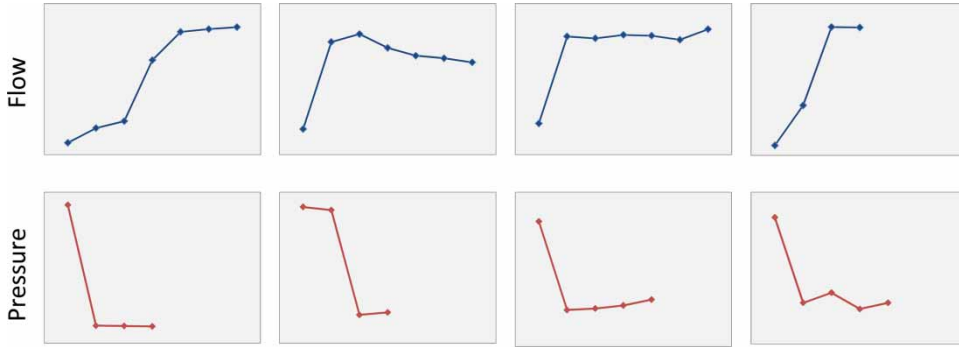
Figure 1 | Burst patterns for WDS hydraulic data (flow top, pressure bottom).
