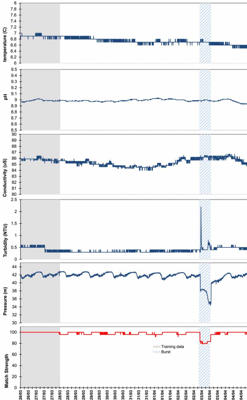
Figure 5 | AURA Alert for abnormal event in water quality data.
