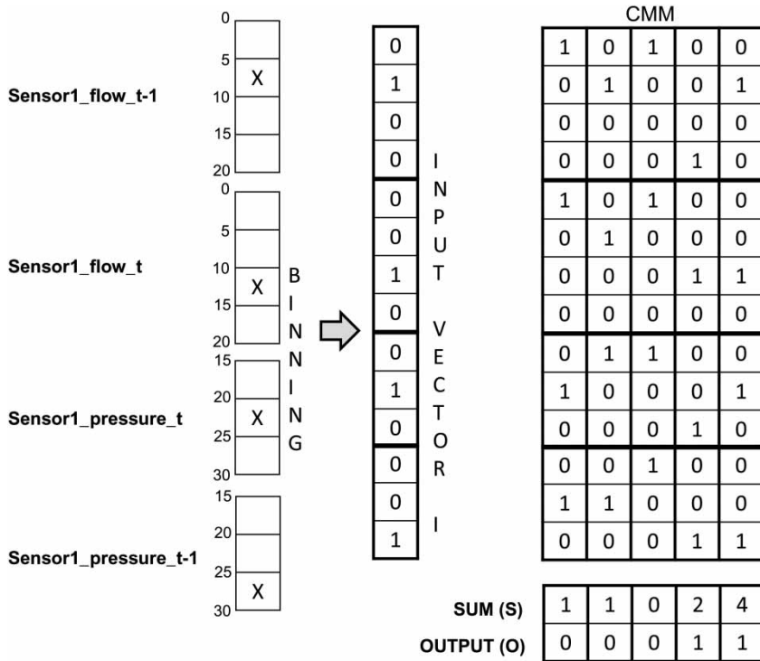
Figure 3 | Input variable binning and the CMM recall process.
