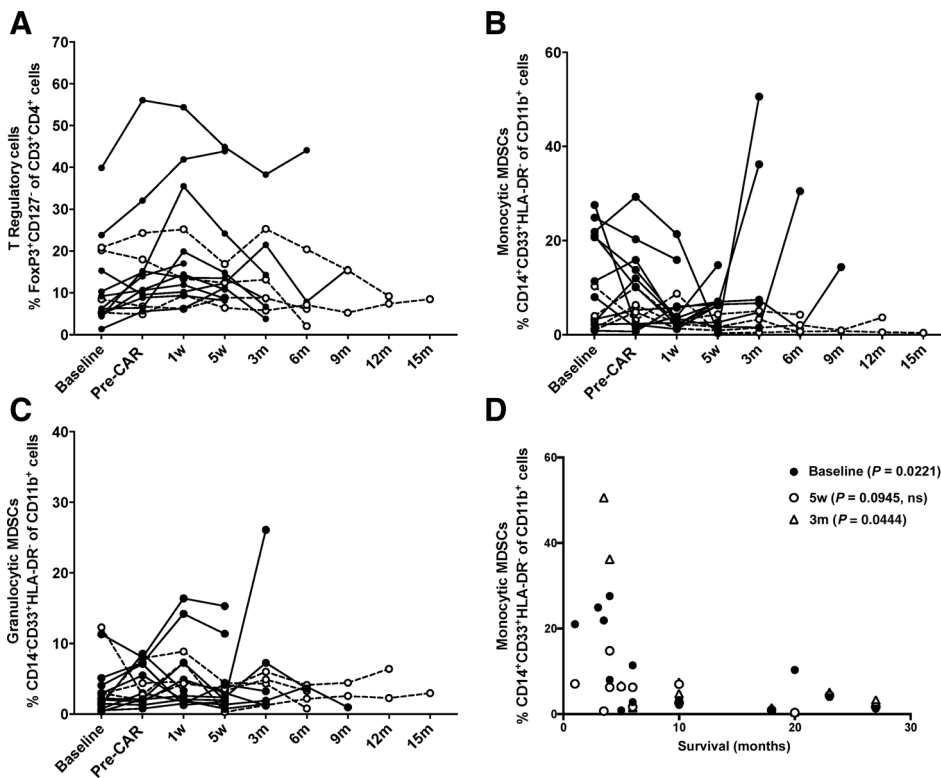
Figure 4. Patients' peripheral blood mononuclear cells were analyzed by flow cytometry for the presence of immunosuppressive cells such as T regulatory cells (A; CD3 + CD4 + CD127-FoxP3 + ), monocytic MDSCs (B; CD14 + CD33 + HLA-DR- of CD11b + ) and granulocytic MDSCs (C; CD14-CD33 + HLA-DR- of CD11b + ). Monocytic MDSCs correlation with survival is shown in D. The samples were analyzed at enrollment (baseline), after conditioning (e.g., day of CAR infusion), and at several time points post treatment (w, week; m, month). Patients still alive are shown as broken lines (no. 2, 5, 6, and 8). Statistical significance was calculated using Spearman correlation test for nonparametric samples.
