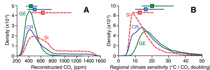
Figure 3. A: Probability density functions (PDFs) for reconstructed CO_2 concentrations from Metasequoia stomatal indices (SI), gas-exchange modeling (GE), and random resampling of the combined stomatal index and gas-exchange model reconstructions (CR). B: PDFs for regional climate sensitivity at the Giraffe locality, subarctic Canada (Appendix DR1 [see footnote 1]). In both panels, horizontal lines indicate the 16 th to 84 th percentile range, with median values marked by squares.
