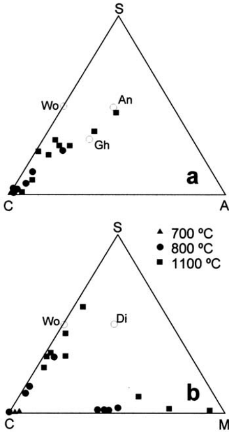
Fig. 6. a) ACS ( \text{Al}_2\text{O}_3\text{-CaO-SiO}_2 ) and b) CMS ( \text{CaO-MgO-SiO}_2 ) compositional diagrams of carbonates and reaction products (EMPA results).
