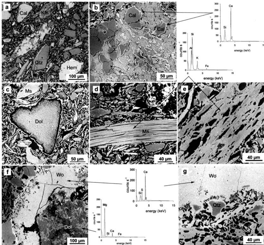
Fig. 5. BSE images and EDX analyses of carbonate-rich Viznar samples: a) fired at 700°C; b) fired at 800°C, when Wo (EDX analysis) formed at the Cal- silicates interface; c) detail of former carbonate grain showing a white outer reaction rim (Wo or Gh?), a crack, and an inner core with an outer darker shell (see text for details); d) Ms (see EDX analysis) at 700°C; e) former Ms after transformation into a Fs? + Mul + melt mixture (see EDX analysis); f) Dol/Phy (+ Qtz) interface showing a reaction rim with fingered geometry formed at 1100°C; g) detail of the outer reaction rim in previous figure; EDX analysis shows the rim composition ( i.e. , Wo).
