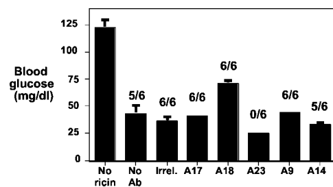
FIGURE 8. In vivo effect of RAC mAbs on ricin toxicity. Mice were injected with 30 µg/kg of ricin holotoxin and 0.8 mg/kg of the indicated Ab. Blood sugar was determined 18 h later. Mice were sacrificed if they became moribund or if their blood sugar level fell below 25 mg/dl. Mean blood sugar levels ( \pm SEM) and survival are shown.
