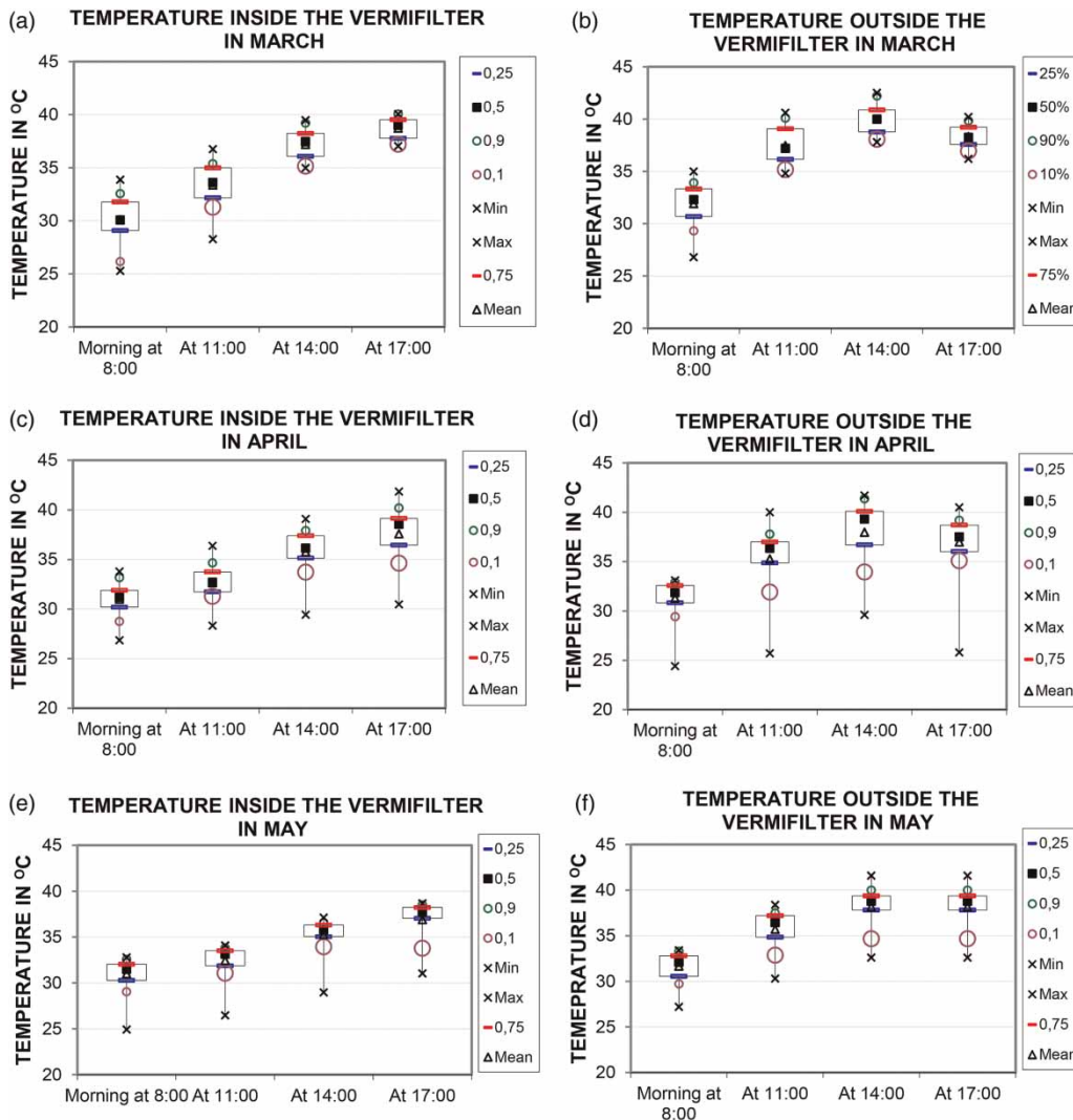
Figure 3 | Average temperature inside the vermifilter (a, c, e) and ambient air temperature outside the vermifilter (b, d, f) in March, April and May.
