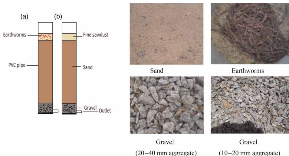
Figure 1 | Filtration system.
