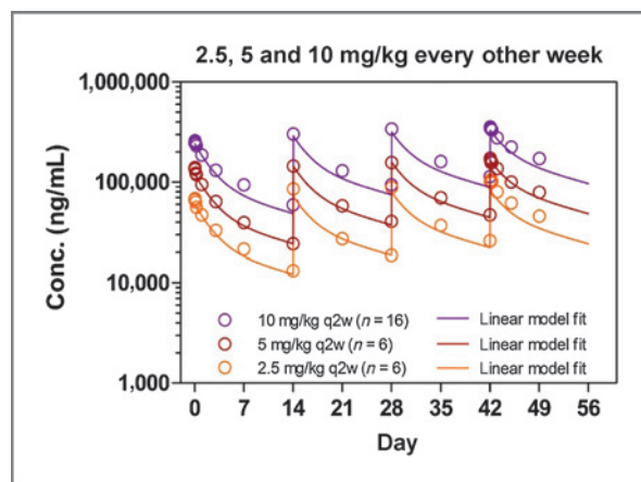
Figure 1. Group mean concentration–time profiles and the linear 2-compartment model fit. Symbols are the observed concentration–time data, by cohort, averaged over nominal time; solid lines are the model predictions by fitting to all the data.
