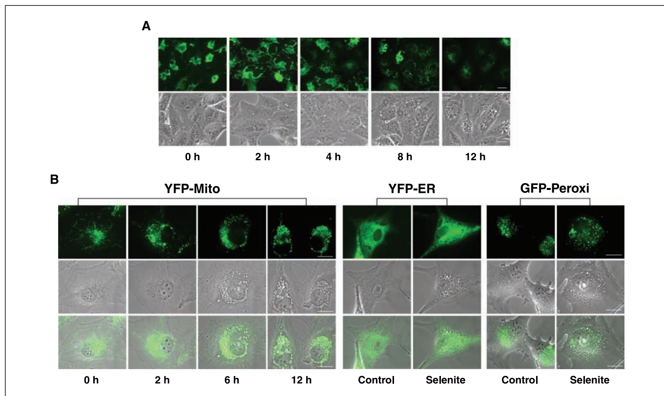
Figure 3. Selenite-induced autophagy is preceded by functional and structural disruption of mitochondria. A , reduction of MMP following selenite treatment. T98G glioma cells were treated with 7 \mu\text{mol/L} selenite for the indicated times and then incubated with Rh-123. Fluorescent and phase-contrast images of cells. Bar, 2 \mu\text{m} . B , mitochondria colocalize with vacuoles induced by selenite treatment, whereas the ER and peroxisomes do not. YFP-Mito cells were treated with 7 \mu\text{mol/L} selenite for the indicated times and observed under a fluorescence microscope. Bar, 2 \mu\text{m} . Fluorescent and phase-contrast images of cells are superimposed. To examine the effect of selenite on ER or peroxisomes, U87MG cell lines stably expressing the pEYFP-ER (YFP-ER cells) or pEGFP-Peroxi (GFP-Peroxi cells) were treated with 7 \mu\text{mol/L} selenite for 12 h and observed under a fluorescence microscope.
