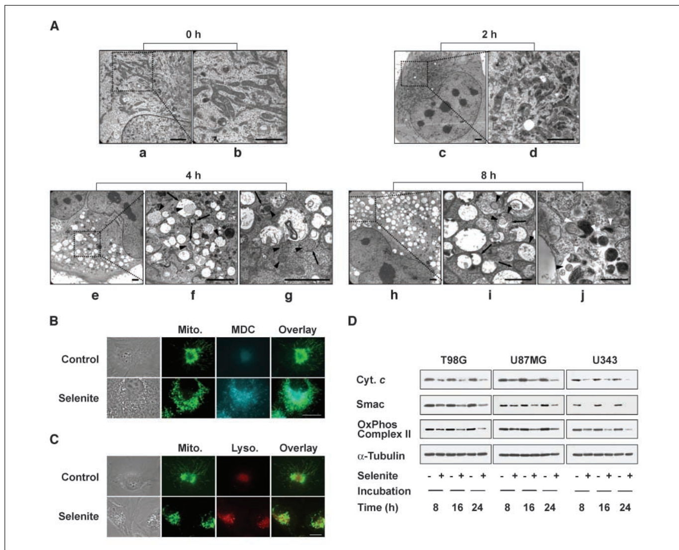
Figure 4. A, electron microscopic observation of glioma cells treated with selenite. T98G cells were untreated or treated with 7 \mu mol/L selenite for the indicated times and transmission electron microscopy was done. Bar, 2 \mu m. B, mitochondria (Mito.) and autophagic vacuoles may fuse after selenite treatment. YFP-Mito cells were untreated or treated with 7 \mu mol/L selenite for 12 h and then incubated with MDC. Changes in mitochondrial morphologies and cellular MDC uptake were observed under a fluorescence microscope. Bar, 2 \mu m. C, mitochondria and lysosomes (Lyso.) may fuse after selenite treatment. YFP-Mito cells were left untreated or treated with 7 \mu mol/L selenite for 12 h and then incubated with LysoTracker Red. Changes in mitochondrial morphologies and lysosomes were observed under a fluorescence microscope. Bar, 2 \mu m. D, reduction of mitochondrial protein levels during selenite-induced cell death. T98G, U87MG, or U343 cells were treated with 7 \mu mol/L selenite for the indicated time points, lysed, and subjected to Western blotting for the indicated mitochondrial proteins. Equal loading of protein samples was confirmed by Western blotting using \alpha -tubulin antibody.
