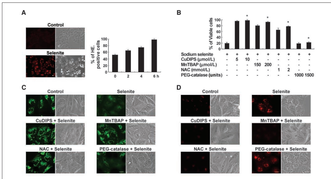
Figure 5. Pretreatment with CuDIPS, MnTBAP, or NAC blocks selenite-induced autophagic cell death. A , generation of superoxide by selenite. T98G cells were treated with 7 \mu\text{mol/L} selenite for 6 h, exposed to hydroethidine, and observed under a fluorescence microscope. Bar, 2 \mu\text{m} ( left ). The accumulation of intracellular superoxide levels was also measured in T98G cells following treatment with selenite for the indicated times and subsequent incubation with hydroethidine (HE) using a fluorescence-activated cell sorter ( right ). B , effect of various antioxidants on selenite-induced cell death. T98G cells were pretreated with the indicated concentrations of antioxidants for 24 h, and cellular viability was assessed using calcein-AM and EthD-1. Columns , average of three independent experiments; bars , SE. *, P < 0.001 , compared with cells treated with selenite. C , pretreatment with CuDIPS, MnTBAP, or NAC blocks selenite-induced loss of MMP. T98G cells were treated with or without 10 \mu\text{mol/L} CuDIPS, 200 \mu\text{mol/L} MnTBAP, 2.5 mmol/L NAC, or 1,000 units PEG-catalase for 30 min, further treated with 7 \mu\text{mol/L} selenite for 8 h, and then incubated with Rh-123. Representative fluorescent and phase-contrast images of cells. Bar, 2 \mu\text{m} . D , pretreatment with CuDIPS, MnTBAP, or NAC blocks selenite-induced AVO formation. T98G cells were pretreated with or without 10 \mu\text{mol/L} CuDIPS, 200 \mu\text{mol/L} MnTBAP, 2.5 mmol/L NAC, or 1,000 units PEG-catalase for 30 min, further treated with 7 \mu\text{mol/L} selenite for 12 h, and then incubated with acridine orange. Representative fluorescent and phase-contrast images of cells. Bar, 2 \mu\text{m} .
