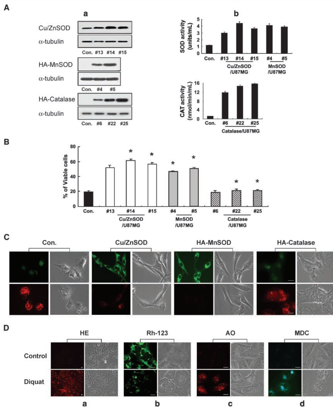
Figure 6. Selenite-induced autophagic cell death is blocked by overexpression of Cu/ZnSOD or MnSOD but not by catalase. A , a , establishment of the stable cell lines overexpressing antioxidant proteins. U87MG cells were stably transfected with expression vectors encoding Cu/ZnSOD, HA-MnSOD, or HA-catalase. As a control, Con. cells (U87MG cells transfected with pcDNA3) were used. Protein levels of the respective antioxidant proteins were analyzed by Western blotting using anti-Cu/ZnSOD or anti-HA antibodies, and equal loading of protein samples was confirmed by Western blotting of \alpha -tubulin. b , Measurement of SOD and catalase (CAT) activity in the established stable cell lines. SOD activity in the lysates from the stable cell lines overexpressing Cu/ZnSOD or MnSOD was measured and compared with that of Con. cells using SOD assay kit (Cayman Chemical Co.). Representative results of three independent experiments. Catalase activity in the lysates from the stable cell lines overexpressing catalase was also compared with that of Con. cells using catalase assay kit (Cayman Chemical Co.). Similar results were obtained from three independent experiments. B , overexpression of SOD, but not catalase, blocks selenite-induced cell death. Con. cells and cells overexpressing Cu/ZnSOD, MnSOD, or catalase were treated with 7 \mu mol/L selenite for 24 h, and cellular viabilities were assessed using calcein-AM and EthD-1. Columns , average of three independent experiments; bars , SE. *, P < 0.001 , compared with cells treated with selenite. C , overexpression of Cu/ZnSOD or MnSOD, but not catalase, blocks selenite-induced loss of MMP and autophagy. Con. cells and cells overexpressing Cu/ZnSOD (clone 15), MnSOD (clone 5), or catalase (clone 25) were treated with 7 \mu mol/L selenite for 8 h and then incubated with Rh-123. Representative fluorescent and phase-contrast images. Bar, 2 \mu m ( top ). The same cells were incubated with 7 \mu mol/L selenite for 12 h and then stained with acridine orange. Representative fluorescent and phase-contrast images. Bar, 2 \mu m ( bottom ). D , generation of superoxide by diquat induces autophagy. For detection of diquat-induced superoxide generation, T98G cells were treated with or without 10 \mu mol/L diquat for 12 h and then stained with hydroethidine. Representative fluorescent and phase-contrast images. Bar, 2 \mu m ( D, a ). For the detection of MMP loss or induction of autophagy, T98G cells were treated with or without 10 \mu mol/L diquat for 16 h and then stained with Rh-123, acridine orange (AO), or MDC. Representative fluorescent and phase-contrast images. Bar, 2 \mu m ( D, b-d ).
