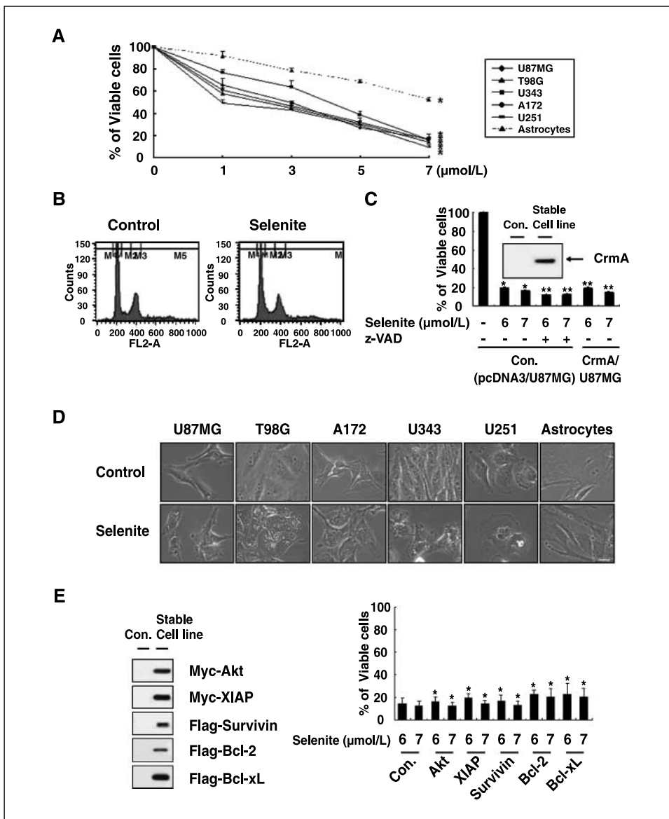
Figure 1. Sodium selenite induces caspase-independent nonapoptotic cell death in various malignant glioma cells but not in normal astrocytes. A , effect of selenite on the viability of human glioma cells and astrocytes. Human glioma cells and astrocytes were treated with the indicated concentrations of selenite for 24 h. Cellular viability was assessed using calcein-AM and EthD-1. Points, mean of three independent experiments; bars, SE. *, P < 0.01, compared with untreated cells. B , DNA content of glioma cells treated with selenite. U87MG cells were untreated or treated with 7 µmol/L selenite for 24 h, and DNA contents were measured by fluorescence-activated cell sorting analysis. C , inhibition of caspases by z-VAD pretreatment or CrmA overexpression does not block selenite-induced cell death. Con. cells (pcDNA3/U87MG; U87MG cells stably transfected with pcDNA3) were pretreated with 50 µmol/L z-VAD-fmk for 30 min and further treated with the indicated concentrations of selenite for 24 h. Cellular viability was assessed using calcein-AM and EthD-1. Stable U87MG cell lines overexpressing CrmA were established and CrmA expression was examined by Western blotting. Con. cells and CrmA-overexpressing U87MG cells were treated with selenite for 24 h, and cellular viabilities were compared using calcein-AM and EthD-1. Columns, average of three independent experiments; bars, SE. *, P < 0.001, compared with untreated cells; **, P < 0.01, compared with cells treated with selenite. D , morphologies of selenite-treated glioma cells and astrocytes. Various glioma cells and astrocytes were treated with 7 µmol/L selenite for 12 h and observed under a phase-contrast microscope. Bar, 2 µm. Representative pictures. E , effects of the overexpression of various antiapoptotic proteins on selenite-induced cell death. Stable cell lines overexpressing Myc-tagged Akt or XIAP, Flag-tagged survivin, Bcl-2, or Bcl-xL were established and their respective overexpressions were confirmed with Western blotting using anti-Myc or anti-Flag antibodies. Con. cells and the respective overexpressing cell lines were treated with 7 µmol/L selenite for 24 h and cellular viabilities were assessed using calcein-AM and EthD-1. Columns, average of three independent experiments; bars, SE. *, P < 0.01, compared with cells treated with selenite. To avoid problems of clonal variability, more than three different subclones of each overexpressing cell line were tested, and similar results were obtained in each case.
