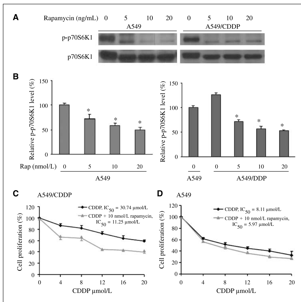
Figure 5. The AKT/mTOR pathway was involved in the chemosensitivity of A549 and A549/CDDP to CDDP treatment.
