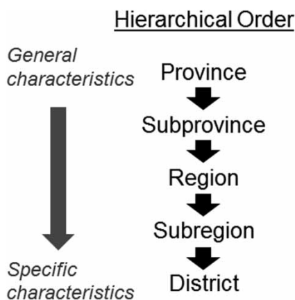
Figure 2 | Hierarchical order used in the hydrogeological regionalization.
