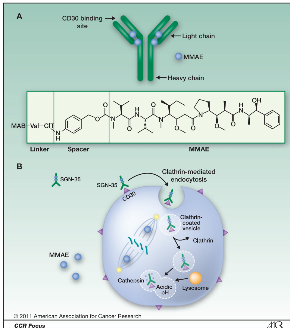
Figure 2. A, SGN-35 structure. MMAE is attached to the IgG1 monoclonal antibody cAC10 by sulfhydryl groups in cysteine residues. A mild reduction of the interchain disulfides is used to attach the citrulline-valine dipeptide linker. A variable number of drug molecules are attached, ranging from 2 to 8, with 4 being the most prevalent. B, ADC internalization process. SGN-35 is internalized following binding to cell surface CD30 by clathrin-mediated endocytosis. The clathrin-coated vesicle is uncoated to allow fusion with lysosomes, and clathrin recirculates to the cell surface. In the acidic milieu of the vesicle, cathepsin cleaves the citrulline-valine dipeptide linker to release free MMAE. MMAE binds to microtubules to prevent mitosis, and free MMAE can diffuse out to the cell to produce cytotoxicity in the tumor microenvironment.
