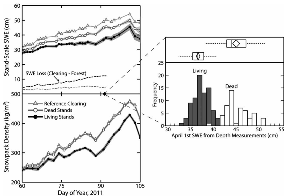
Figure 3 | Stand-scale SWE and snowpack density graphed against Day of Year, 2011. Dot markers in SWE and density graphs represent average measurements, and shaded regions represent 95% confidence intervals. SWE Loss in the stand-scale SWE graph was calculated as reference clearing SWE minus forest SWE. A histogram of snow depth values in living and dead forest stands for 1 April with average, maximum, median, minimum and quartile distribution values is inset.
