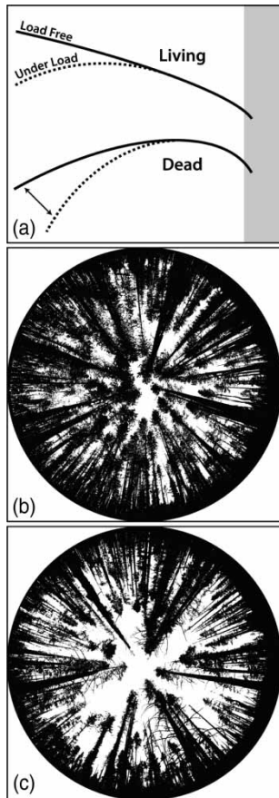
Figure 6 | (a) Branch shape and deflection commonly observed in living and grey phase dead lodgepole pine found in north-central Colorado. Hemispherical photographs of two lodgepole pine stands with similar basal area. (b) A living stand with an LAI' value of 1.29 and (c) a grey phase dead stand with an LAI' value of 0.73.
