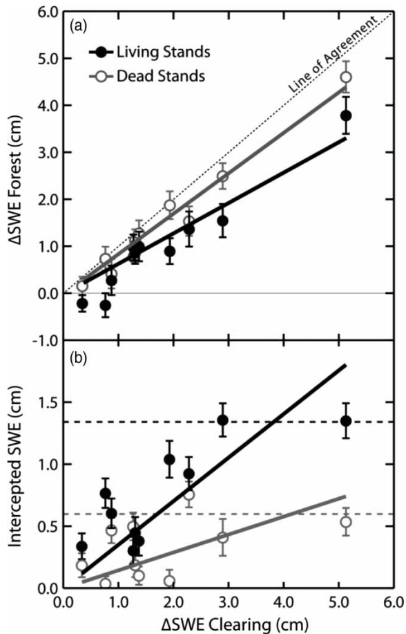
Figure 4 | (a) Event (storm) snowfall SWE: forest subcanopy versus clearing SWE for living ( y = 0.64x ; p < 0.0001 ; r^2 = 0.89 ) and dead ( y = 0.86x ; p < 0.0001 ; r^2 = 0.97 ) stands. (b) Event (storm) forest intercepted SWE versus clearing SWE ( p < 0.001 ; r^2 = 0.40 ) for living and dead stands ( p = 0.175 ; r^2 = 0.02 ). Error bars represent one standard deviation and dashed lines are average maximum observed interception values (Living = 1.35 cm; Dead = 0.56 cm). Regressions were performed assuming zero subcanopy accumulation when zero clearing accumulation (i.e., forcing the y-intercept of linear regression lines through the origin).
