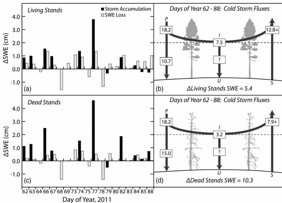
Figure 5 | Water fluxes during the interval DoY 62–88. (a) Storm accumulation and SWE Loss in living stands. (b) Water mass balance in living stands, represented as cm SWE. (c) Storm accumulation and SWE Loss in dead stands. (d) Water mass balance in dead stands, represented as cm SWE. P indicates precipitation, I indicates interception, U indicates unloading and S indicates sublimation.
