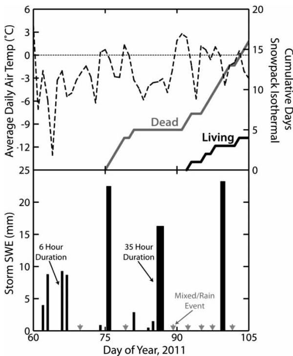
Figure 2 | Average 2-m air temperatures, cumulative days when snowpacks were isothermal in living and dead stands, and storm size reported by Day of Year, 2011. Storms where air temperatures were less than -3 °C are shown in black lines (those included in our analysis); other storms are indicated with grey arrows. Storm size column widths vary with storm duration. Clearing snowpacks became isothermal at the same times as snowpacks under dead canopies.
