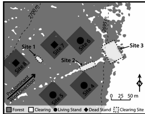
Figure 1 | Site locations along the headwaters of the Colorado River in north-central Colorado. Circle markers represent living stands, diamonds represent grey phase dead stands, and clearing sites are boxed in dashed lines. Shaded areas surrounding stand markers represent stand-scale experimental zones. During the study period, wind direction was predominantly from the southwest (73% of the time).
