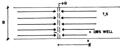
Fig. 3. Auxiliary hydraulic system for calculating the hydraulic properties of an esker.
