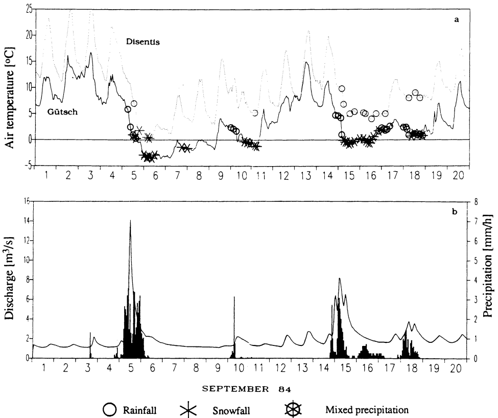
Fig. 3. a) The course of air temperature and observations of the aggregational state of precipitation at the ANETZ stations Gütsch (2,282 m a.s.l.) and Disentis (1,190 m a.s.l.) 1-20 September 1984.
