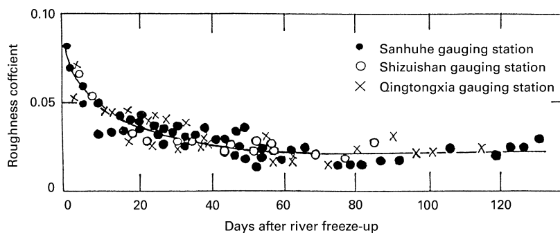
Figure 16 Variation of roughness coefficient of ice jam with time (three gauge stations on the Yellow River)
