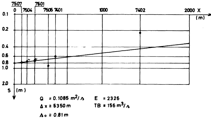
Fig. 14. Evaluation of the hydraulic properties at steady state.
