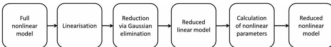
Figure 2 | The model reduction algorithm.
