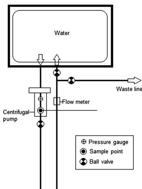
Figure 1 | Diagram of experimental set-up.
