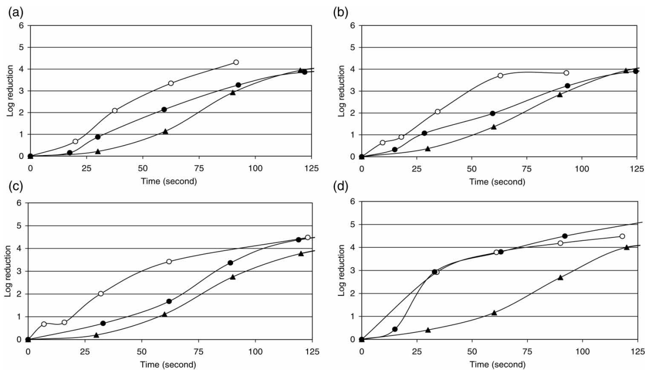
Figure 3 | Bacterial reduction by the UV and the UV/ H_2O_2 processes in waters containing 2 \text{ mg l}^{-1} fulvic acid. (a) H_2O_2 = 0 \text{ mg l}^{-1} , (b) H_2O_2 = 10 \text{ mg l}^{-1} , (c) H_2O_2 = 25 \text{ mg l}^{-1} , and (d) H_2O_2 = 50 \text{ mg l}^{-1} ; key: \circ — Escherichia coli , \bullet — Pseudomonas aeruginosa , \blacktriangle — Bacillus subtilis .
