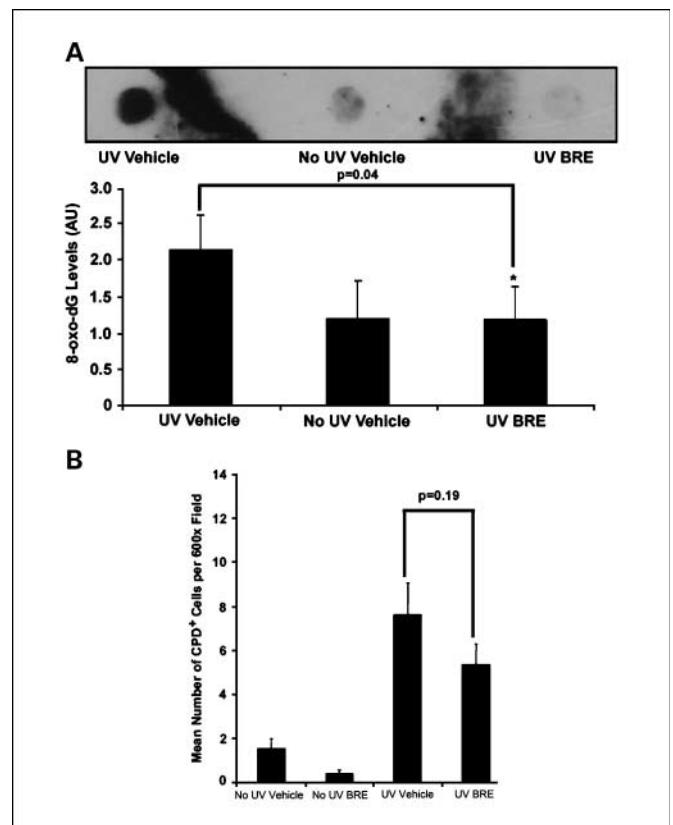
Fig. 6. BRE reduced ROS-mediated DNA damage, but not direct DNA damage. After flash-freezing, DNA was isolated from epidermal scrapes and used in a Southwestern immunoblot (A). Densitometry was done using ImageJ. Columns, ratio of DNA to 8-oxo-dG (8-oxo-dG levels); bars, SD (*, P = 0.04 ); (B). Paraffin sections were cut and stained for CPDs; keratinocytes staining positive were enumerated. Columns, mean number of CPD-positive cells per ×600; bars, SD (C).
