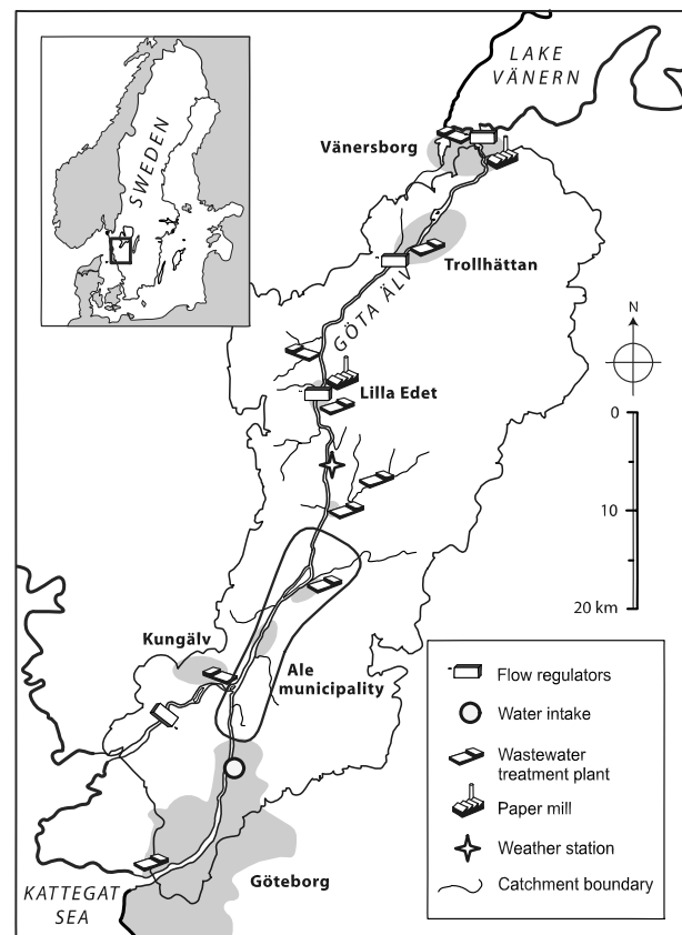
Figure 1 | The river Göta älv and its lower catchment area with the location of wastewater treatment plants, paper mills, weather station and the drinking water intake for Göteborg. The administrative border of the municipality of Ale is marked by a bold line.
