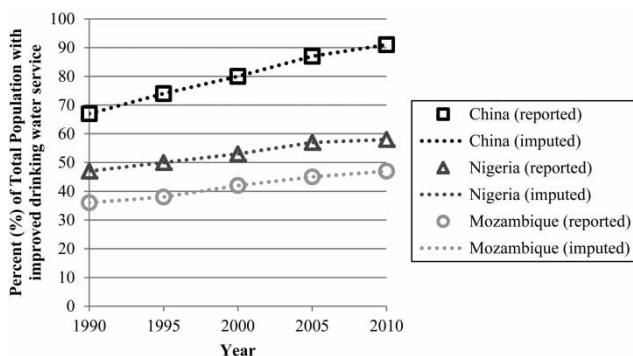
Figure 1 | Illustrative example of the two variants of the drinking water services variable, the reported values ( Water_{total} ), and imputed values ( Water_{total,imputed} ) for three countries (China, Nigeria, and Mozambique) over the years 1990 to 2010.
