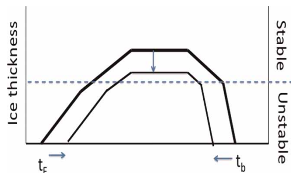
Figure 6 | The influence of climate warming on an ice season. Freezing and break-up dates t_F and t_b come closer to each other. Ice thickness decreases and that reduces the length of the stable ice cover period.
