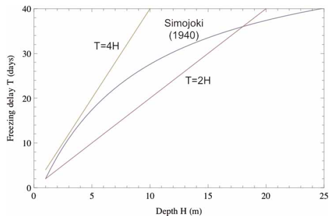
Figure 2 | Delay of the freezing date from the air temperature downcrossing of 0 \text{ } ^\circ\text{C} as a function of the mixed layer depth ( H ) of the lake. The empirical curve of Simojoki (1940) is shown together with lines T[\text{days}] = 2H[\text{m}] and 4H[\text{m}] .
