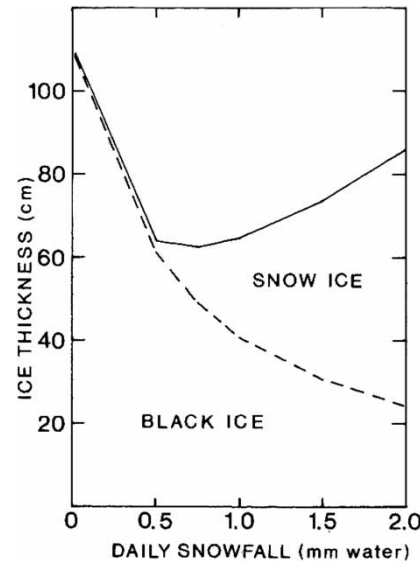
Figure 3 | Thickness of ice calculated with climatological air temperature (Oulu, Finland; 65.0° N, 25.5° E) as a function of daily snowfall (Leppäranta 1983). The solid line presents the total ice thickness, and the dashed line gives the proportions of congelation ice (black ice) and snow-ice.
