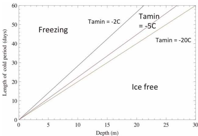
Figure 1 | Freezing conditions for lakes as a function of the lake depth and length of the cold period ( T_a < 0 \text{ } ^\circ\text{C} ).
