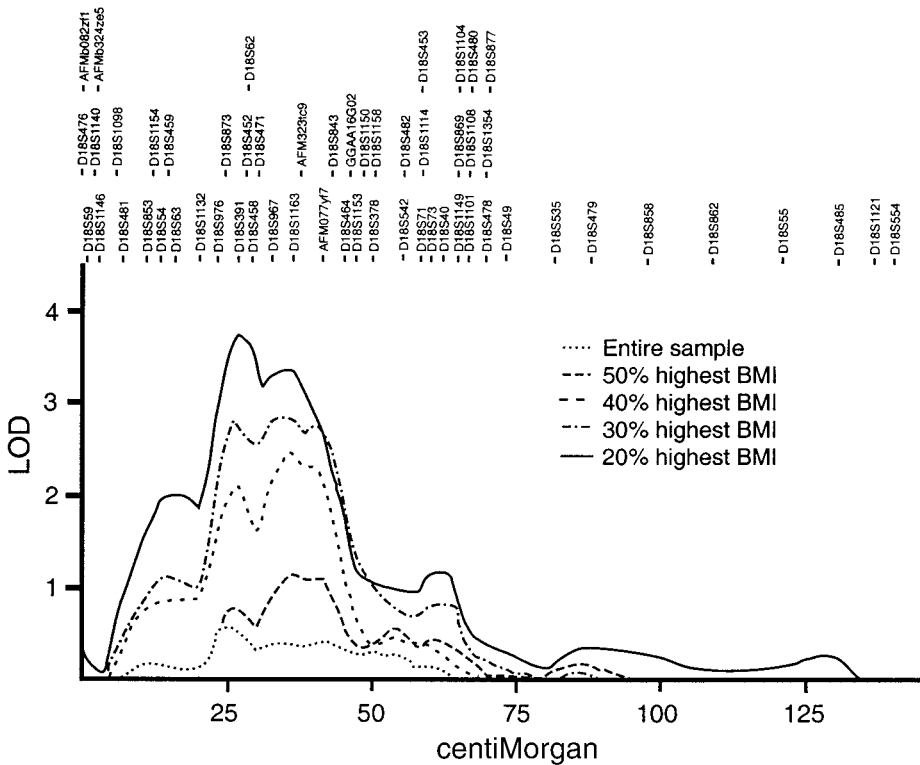
FIG. 2. Reanalysis of chromosome 18 using a 56-marker map.
