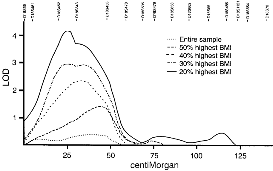
FIG. 1. Multipoint allele sharing analysis of the type 2 diabetes phenotype, stratified by pedigree mean age- and sex-adjusted BMI, using a 15-marker chromosome 18 framework map.
